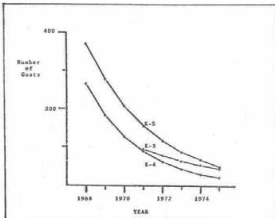
Figure 2. Trends in 3 mountain goat populations near Ketchikan, Alaska, 1968 - 1975, based on the highest pre-decline count and calculated \bar{r} values.
