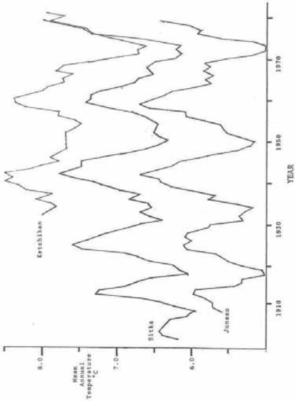
Figure 5. Trends in mean annual temperature at Juneau and Sitka since 1900 (from Juday (1982)) and Ketchikan, Alaska since 1950.
